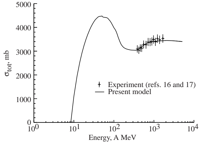
Figure 6. Total cross sections for proton-uranium collision as function of energy.
